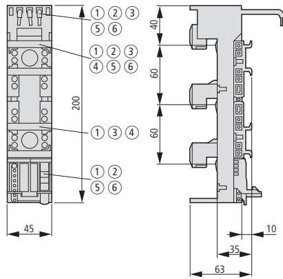
BBA0C-16
