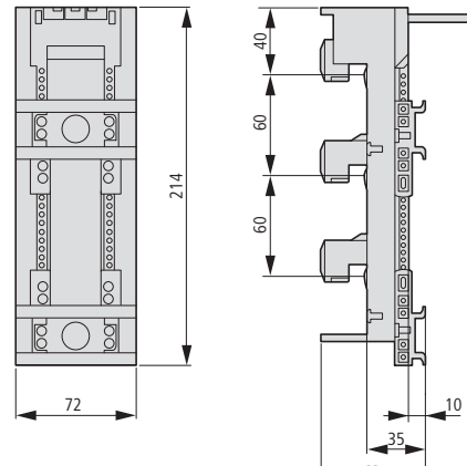
BBA2-80/2TS-S
