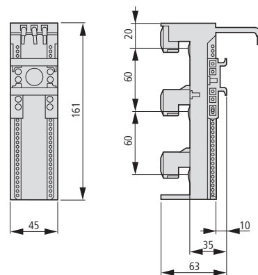
BBA0K-32
