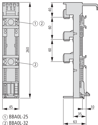
BBA0L-32
