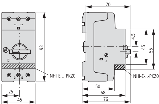
Motor-protective circuit-breaker Transformer-protective circuit-breakers Motor-protective circuit-breaker with standard auxiliary contacts PKZM0...(+NHI-E-...-PKZ0) PKZM0...-T(+NHI-E-...-PKZ0) PKM0...(+NHI-E-...-PKZ0)
