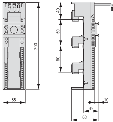
BBA4-63
